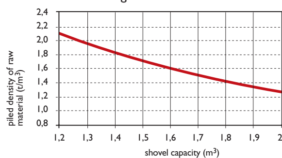
Diagram for shovel selection
